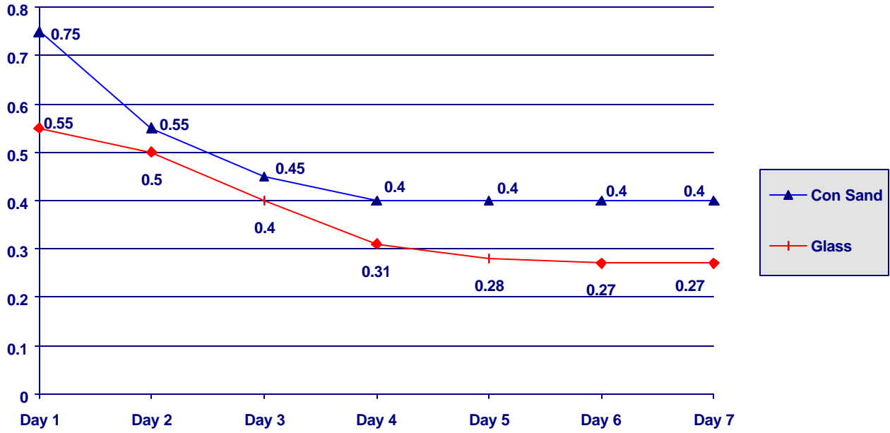
Comparison of Average Turbidity in National Turbidity Units (NTUs)
