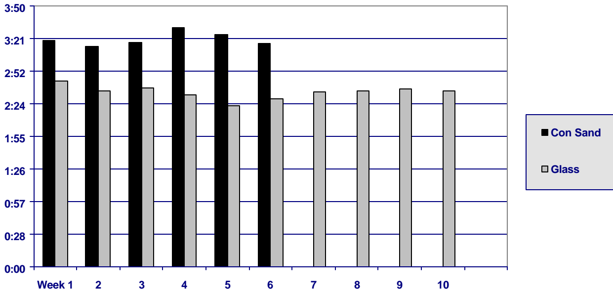
Comparison of Average Backwash Time in Minutes
