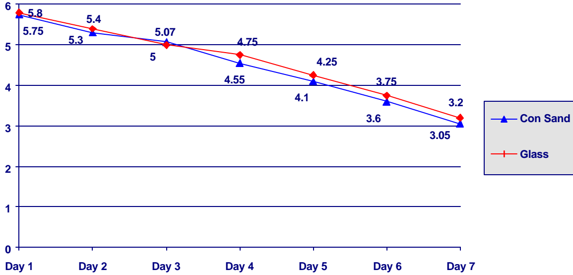
Comparison of Average Effluent Filter Pressures (pounds per square inch)
