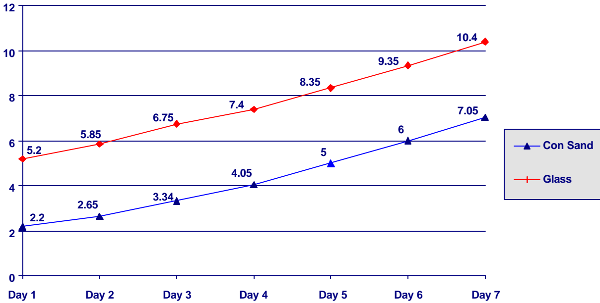
Comparison of Average Differential Filter Pressures (pounds per square inch)
