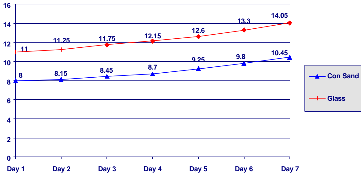
Comparison of Average Influent Pressures (pounds per square inch)
